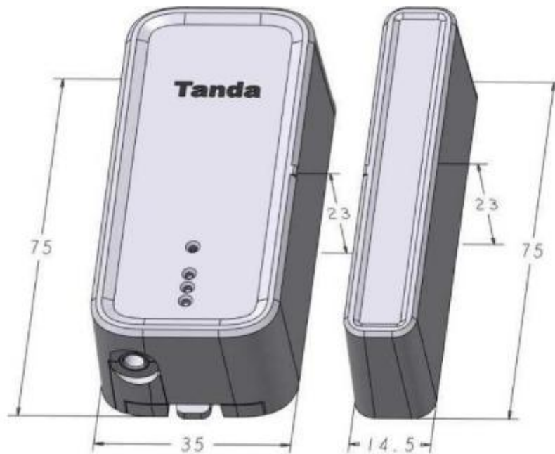
Figure 1 Diagram of TW3207 (Foslink) of outline dimension and installation dimension
