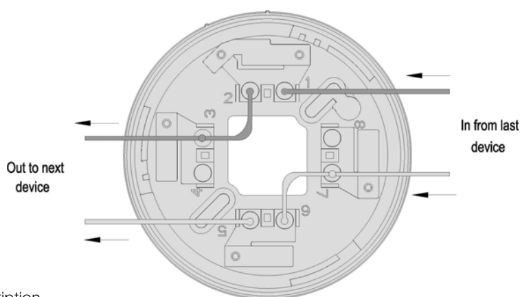
Figure 2: Loop Powered
